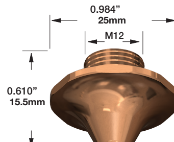
Nozzle EAB
