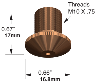
Nozzle 968-41-93-761 1.7mm
