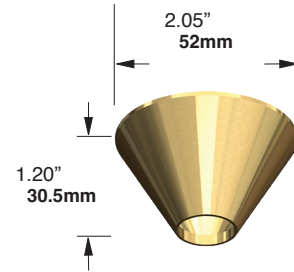
Housing, Water 216-20717
