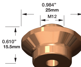
Nozzle EAC
