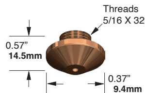
Nozzle 922464 .060" 922465 .080" 922770 .100"
