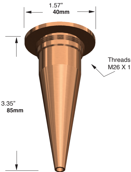
Beam Cone 100.703.5
